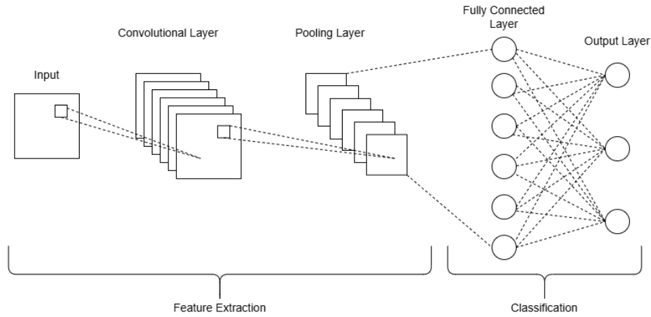
Figure 2.3: CNN Architecture
